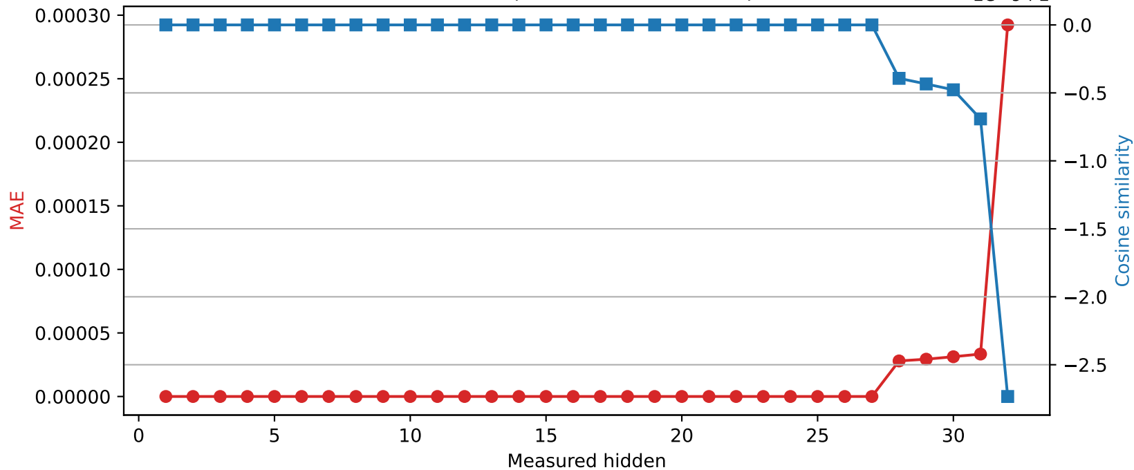
Mistral-7B-Instruct-v0.3 | Quantized layer 27 | float64 → int16
