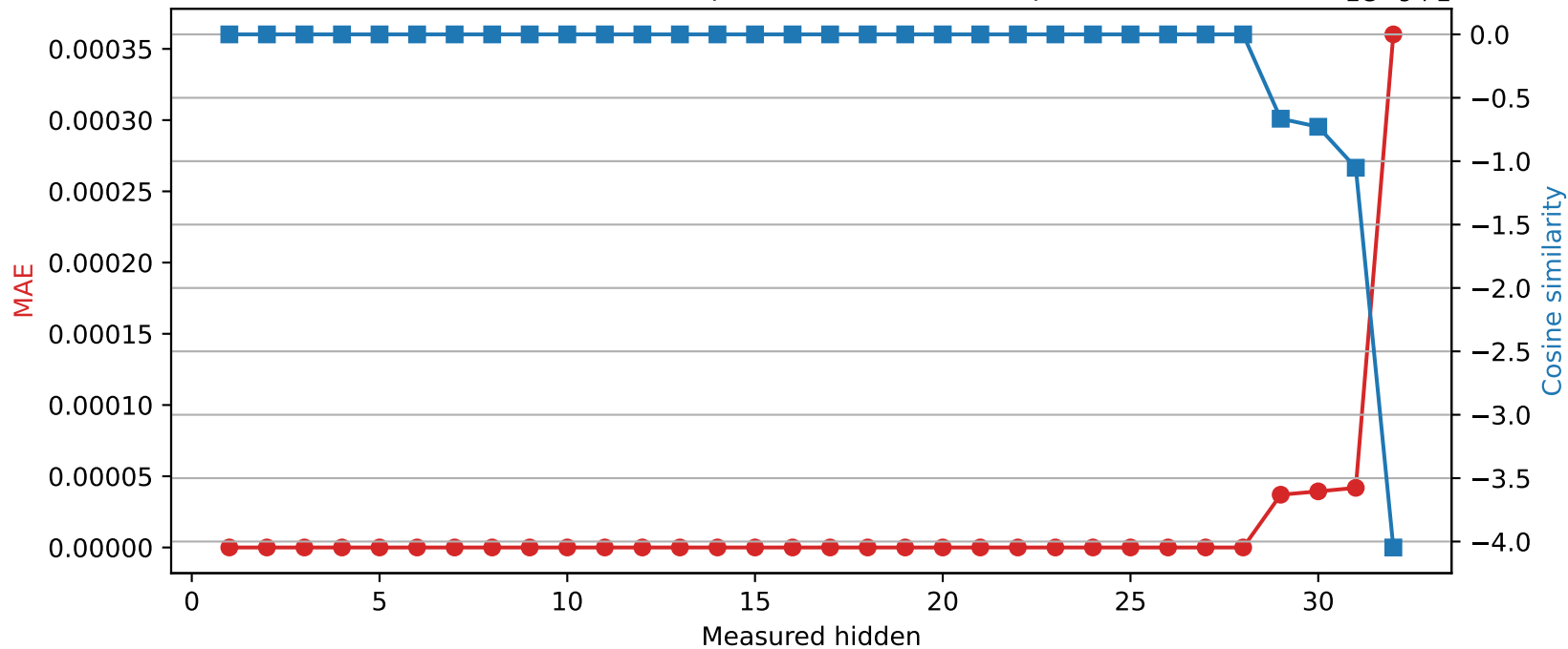
Mistral-7B-Instruct-v0.3 | Quantized layer 28 | float64 → int16
