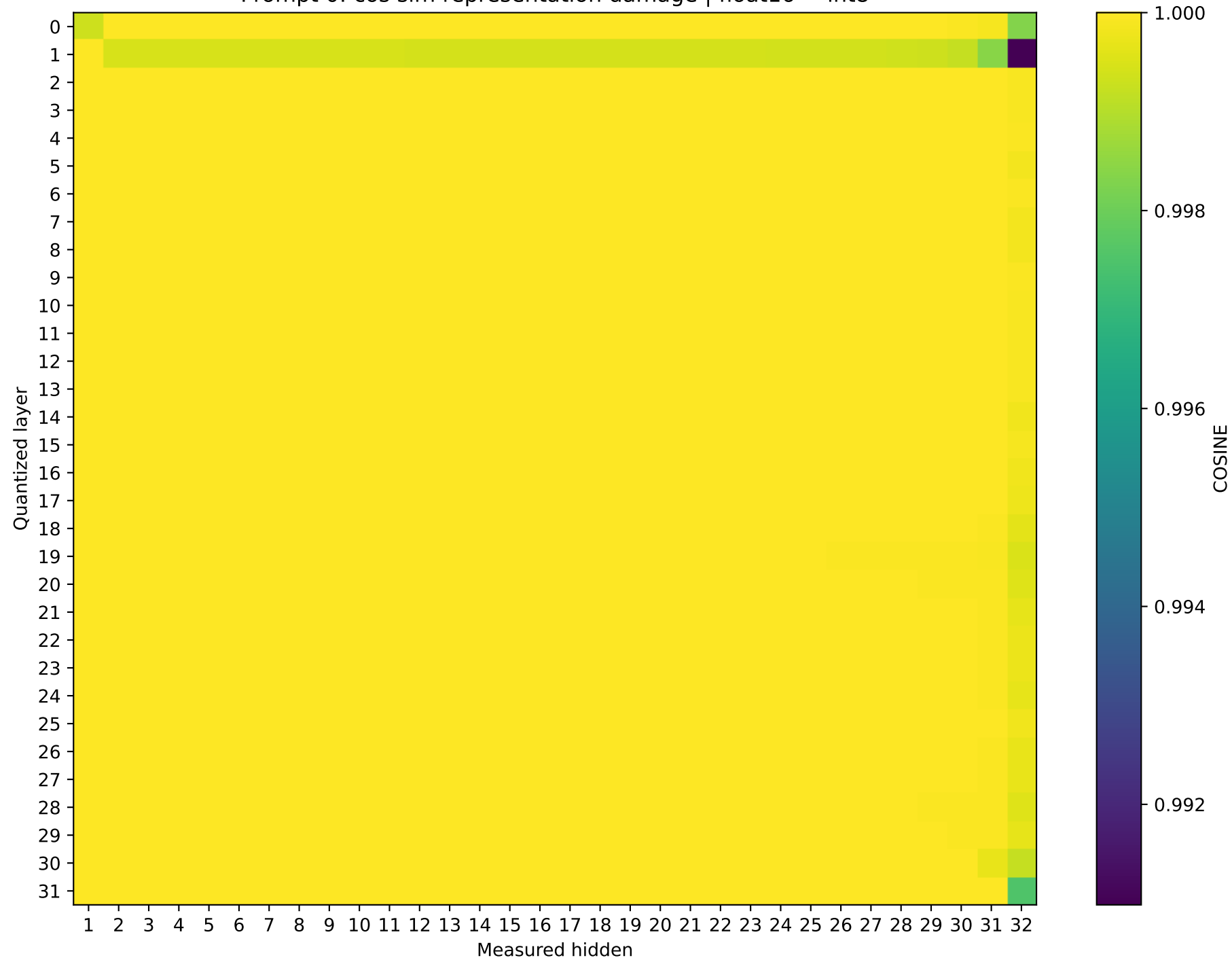
Mistral-7B-Instruct-v0.3 Prompt 0: cos sim representation damage | float16 \rightarrow int8
