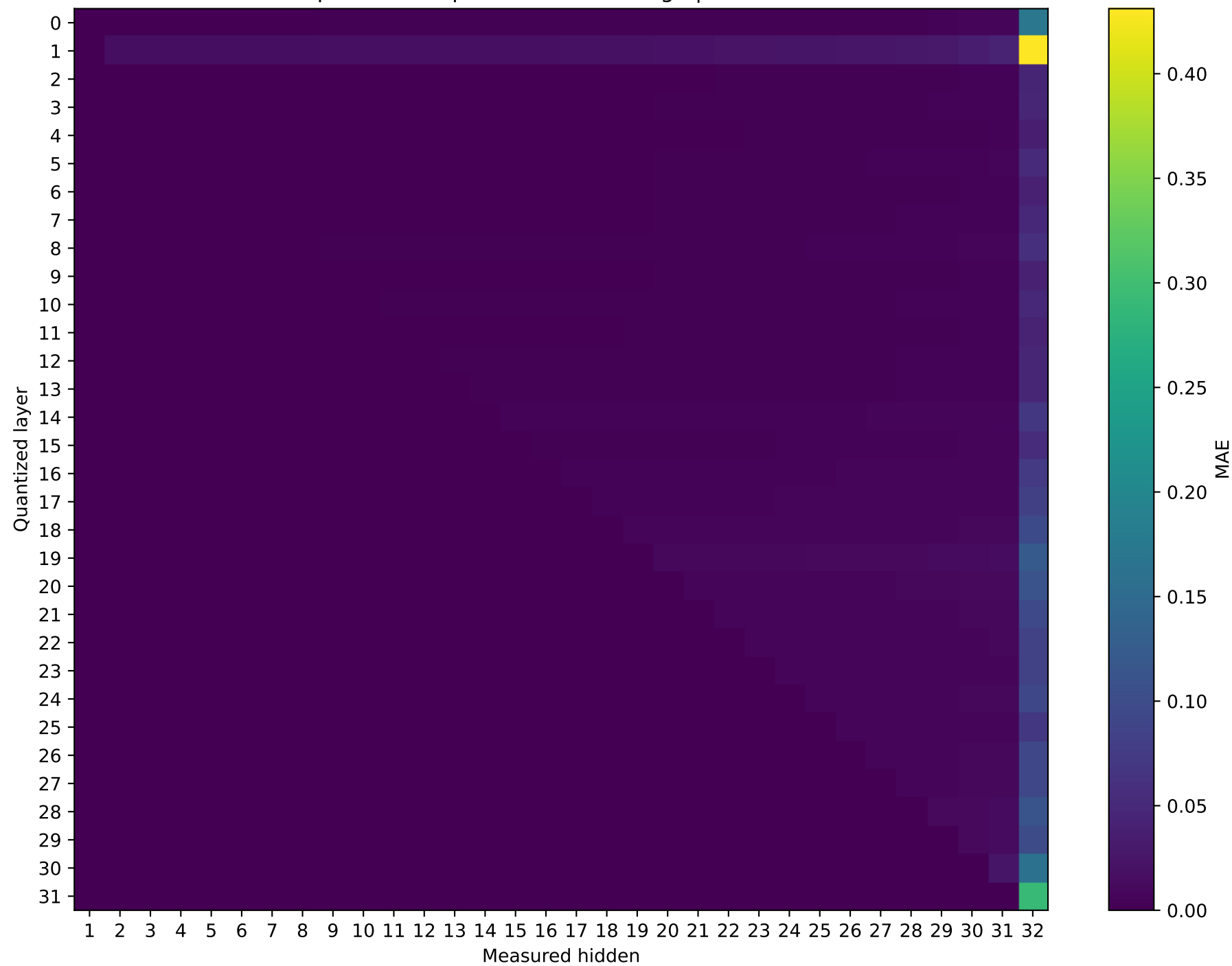
Mistral-7B-Instruct-v0.3 Prompt 0: MAE representation damage | float16 → int8
