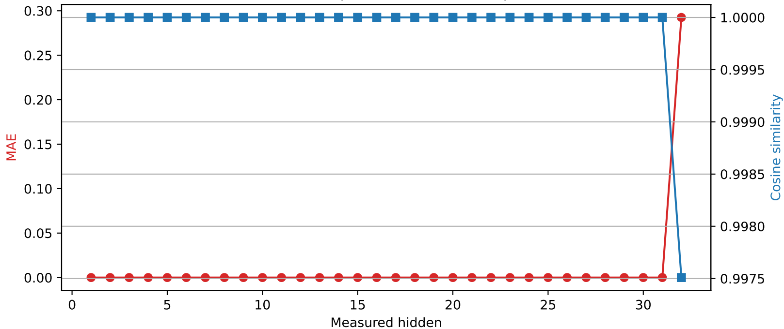
Mistral-7B-Instruct-v0.3 | Quantized layer 31 | float16 → int8
