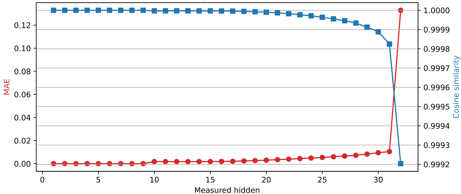
Mistral-7B-Instruct-v0.3 | Quantized layer 9 | float16 → int8
