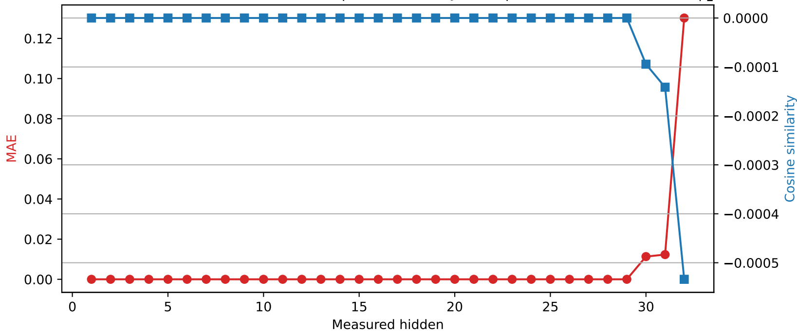
Mistral-7B-Instruct-v0.3 | Quantized layer 29 | float16 \rightarrow int8
