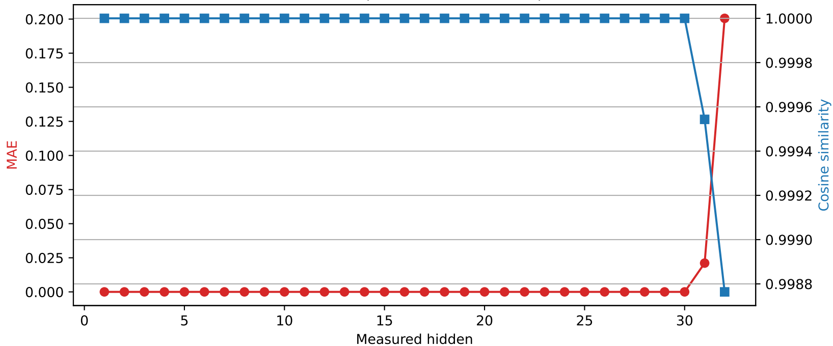
Mistral-7B-Instruct-v0.3 | Quantized layer 30 | float16 → int8
