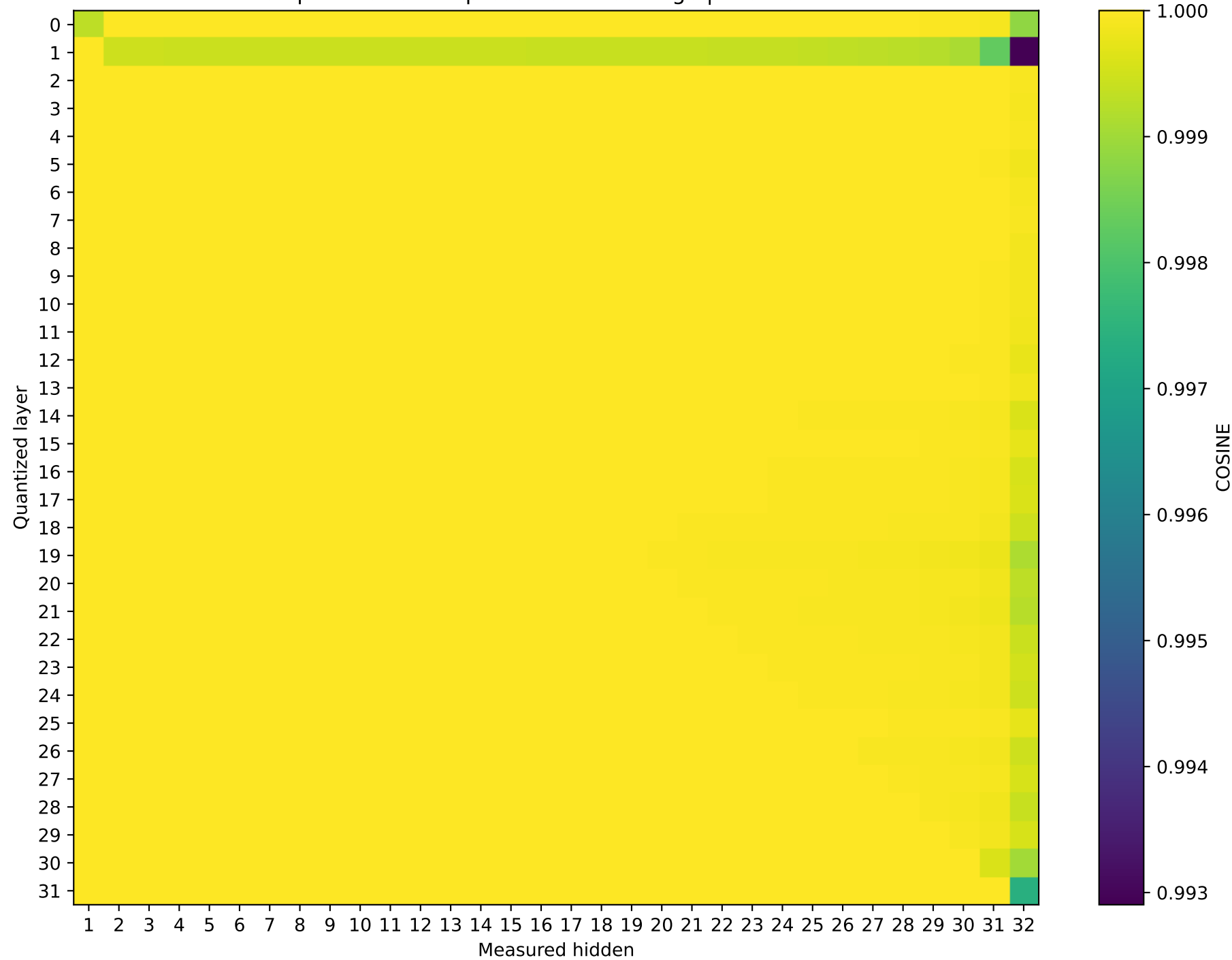
Mistral-7B-Instruct-v0.3 Prompt 2: cos sim representation damage | float16 → int8
