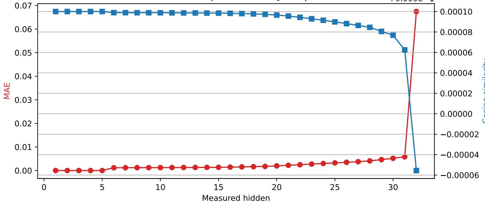
Mistral-7B-Instruct-v0.3 | Quantized layer 5 | float16 → int8
