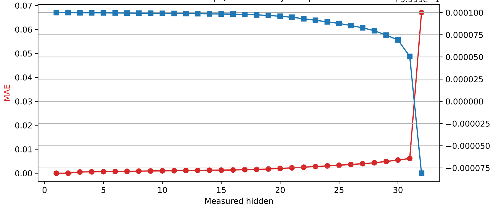
Mistral-7B-Instruct-v0.3 | Quantized layer 2 | float16 \rightarrow int8
