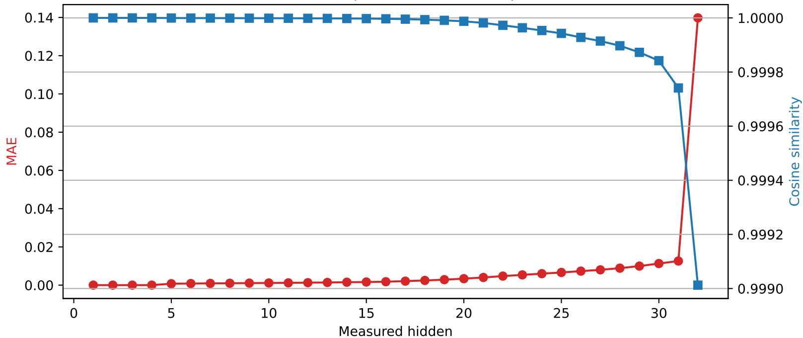
Mistral-7B-Instruct-v0.3 | Quantized layer 4 | float16 \rightarrow int8
