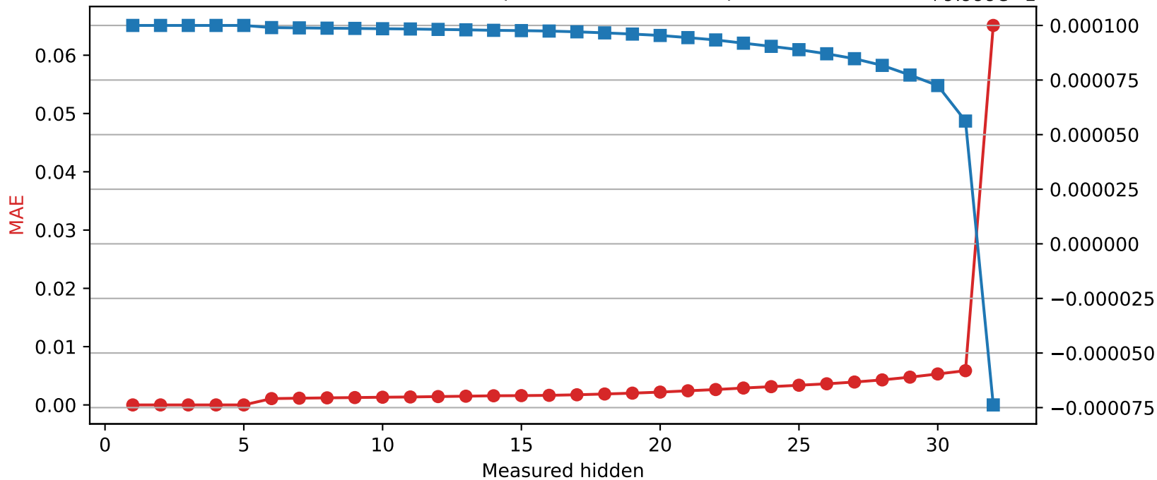
Mistral-7B-Instruct-v0.3 | Quantized layer 5 | float16 \rightarrow int8
