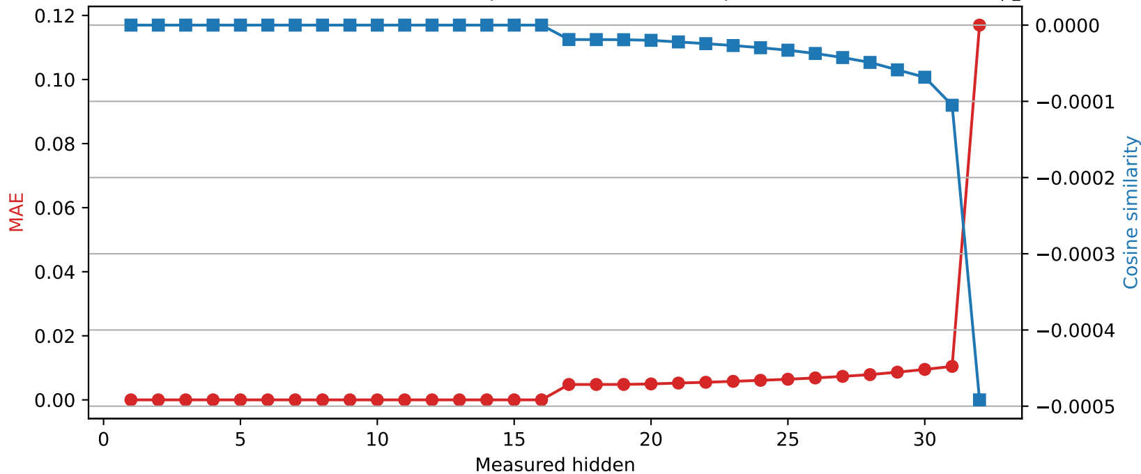
Mistral-7B-Instruct-v0.3 | Quantized layer 16 | float16 → int8
