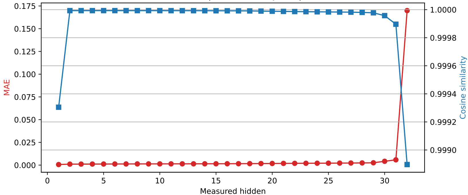
Mistral-7B-Instruct-v0.3 | Quantized layer 0 | float16 → int8
