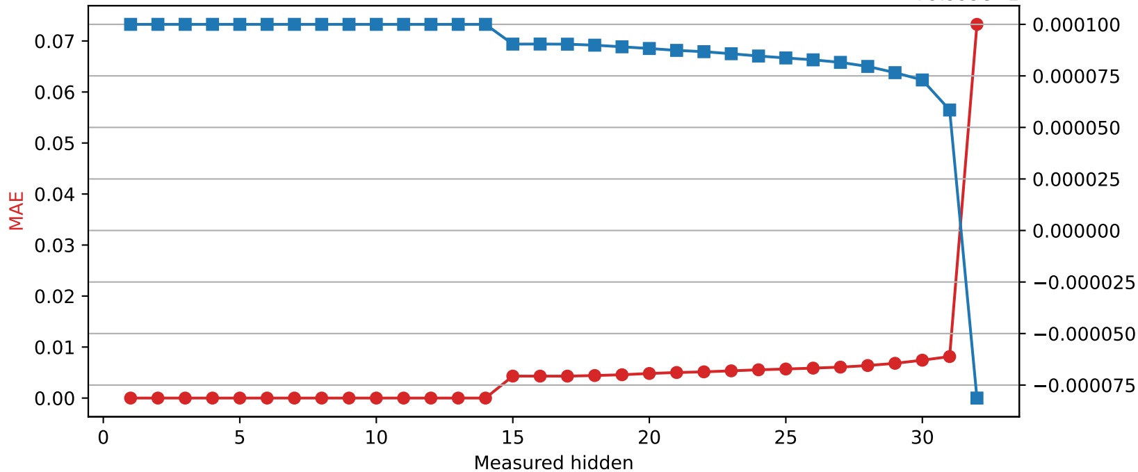
Mistral-7B-Instruct-v0.3 | Quantized layer 14 | float16 → int8 +9.999e-1
