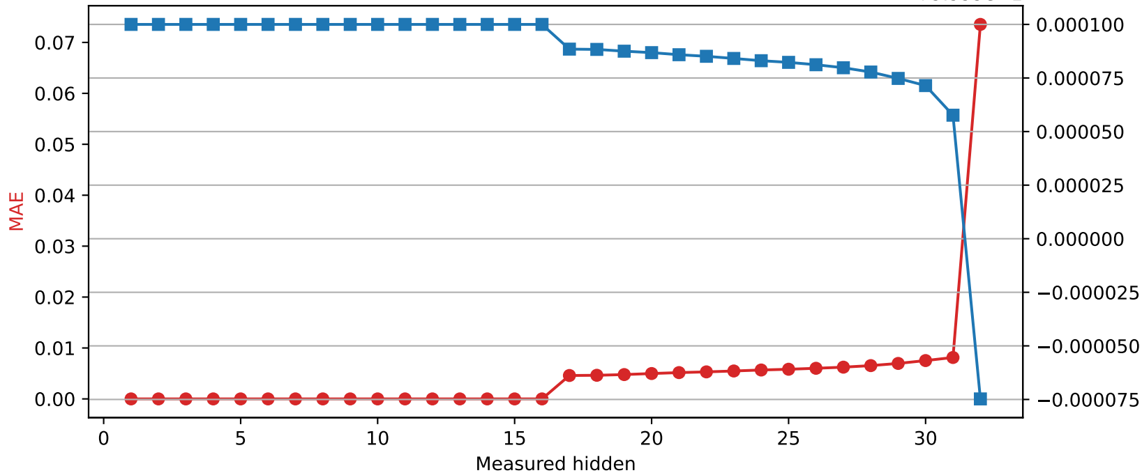
Mistral-7B-Instruct-v0.3 | Quantized layer 16 | float16 → int8 +9.999e-1
