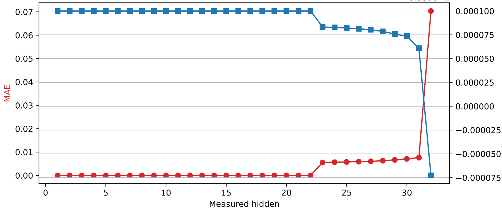
Mistral-7B-Instruct-v0.3 | Quantized layer 22 | float16 → int8 +9.999e-1
