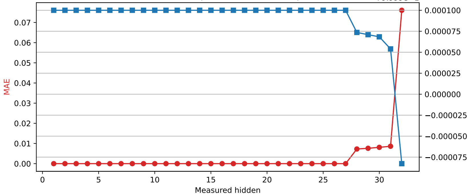
Mistral-7B-Instruct-v0.3 | Quantized layer 27 | float16 \rightarrow int8 +9.999e-1
