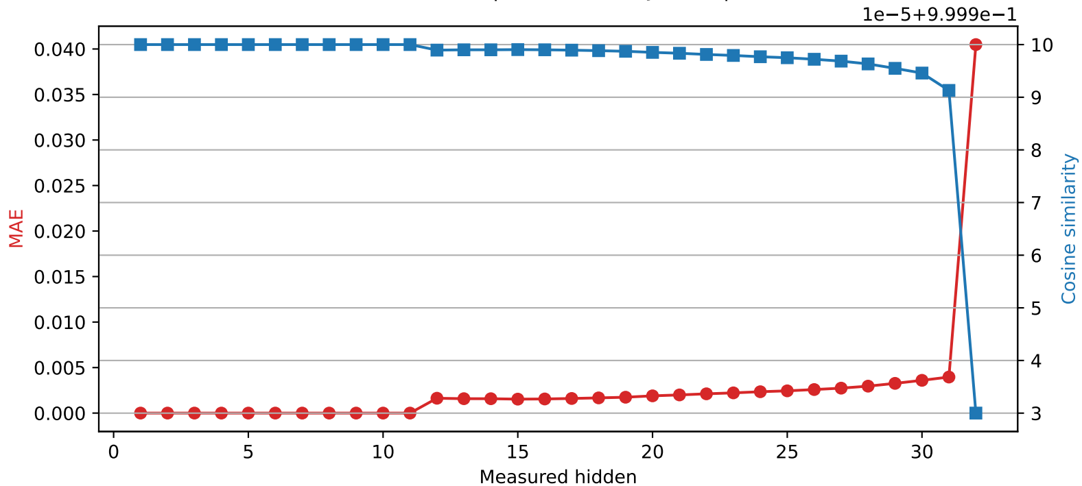
Mistral-7B-Instruct-v0.3 | Quantized layer 11 | float32 → int8
