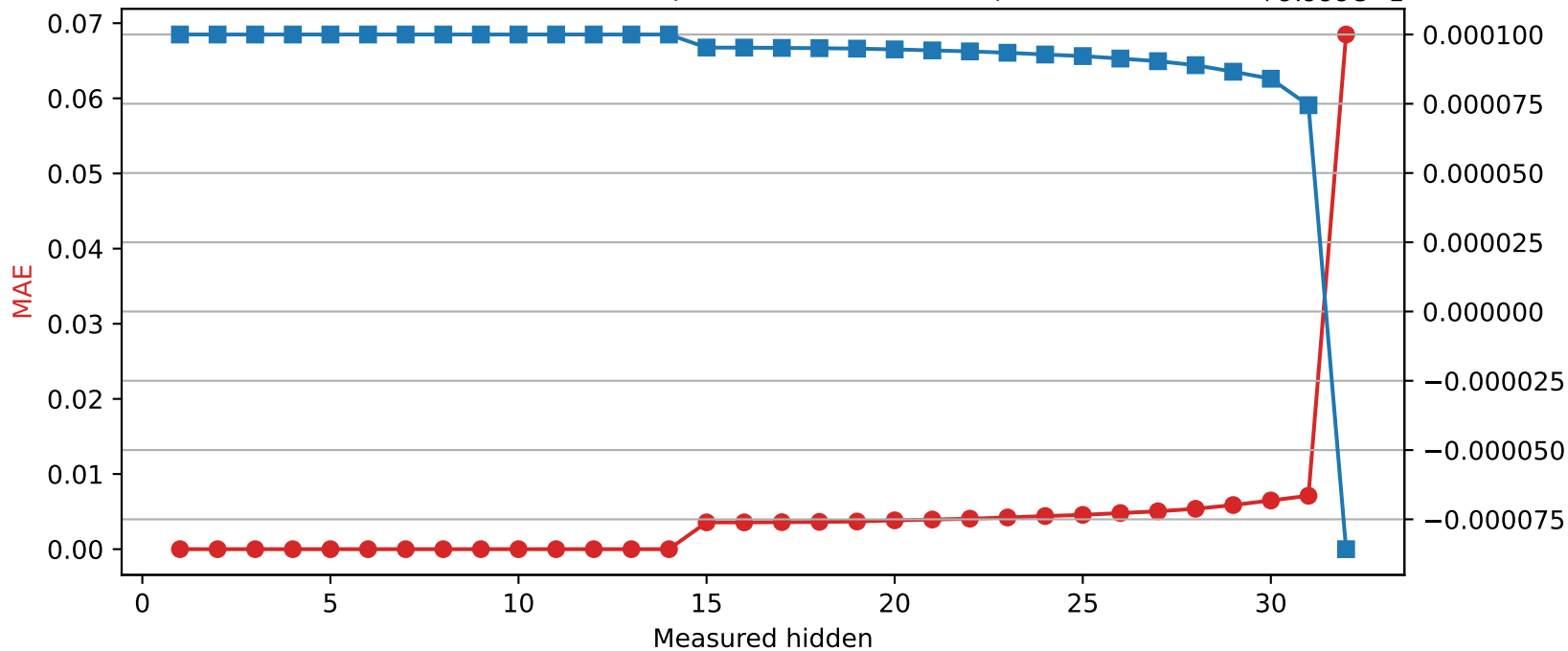
Mistral-7B-Instruct-v0.3 | Quantized layer 14 | float32 \rightarrow int8 +9.999e-1
