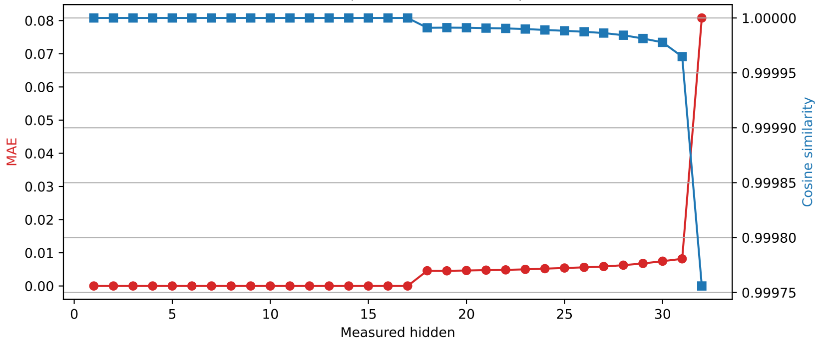
Mistral-7B-Instruct-v0.3 | Quantized layer 17 | float32 \rightarrow int8
