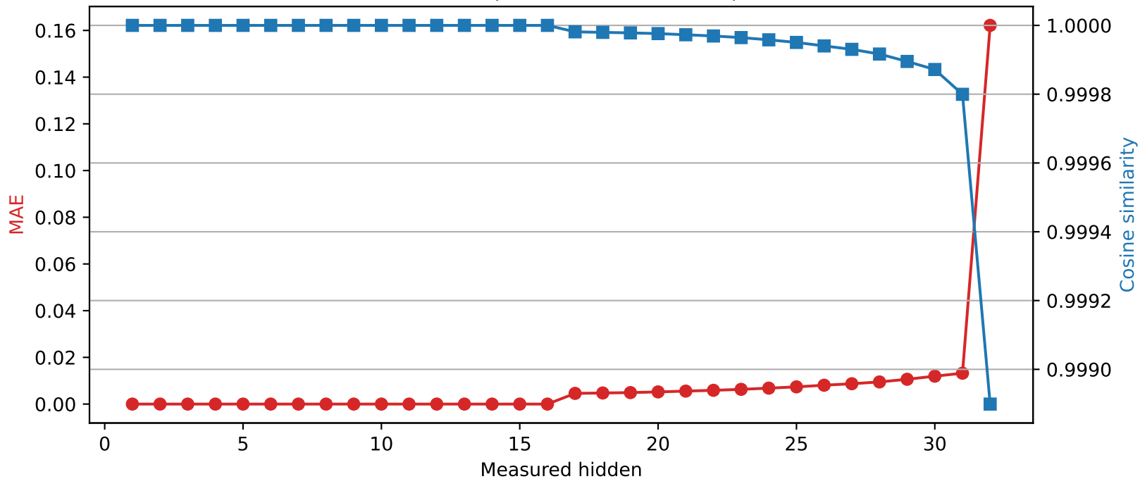
Mistral-7B-Instruct-v0.3 | Quantized layer 16 | float32 → int8
