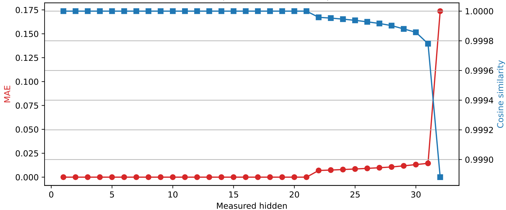
Mistral-7B-Instruct-v0.3 | Quantized layer 21 | float32 → int8
