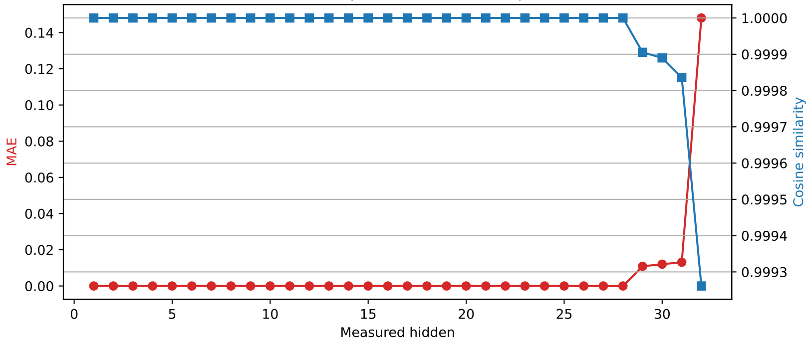
Mistral-7B-Instruct-v0.3 | Quantized layer 28 | float32 → int8
