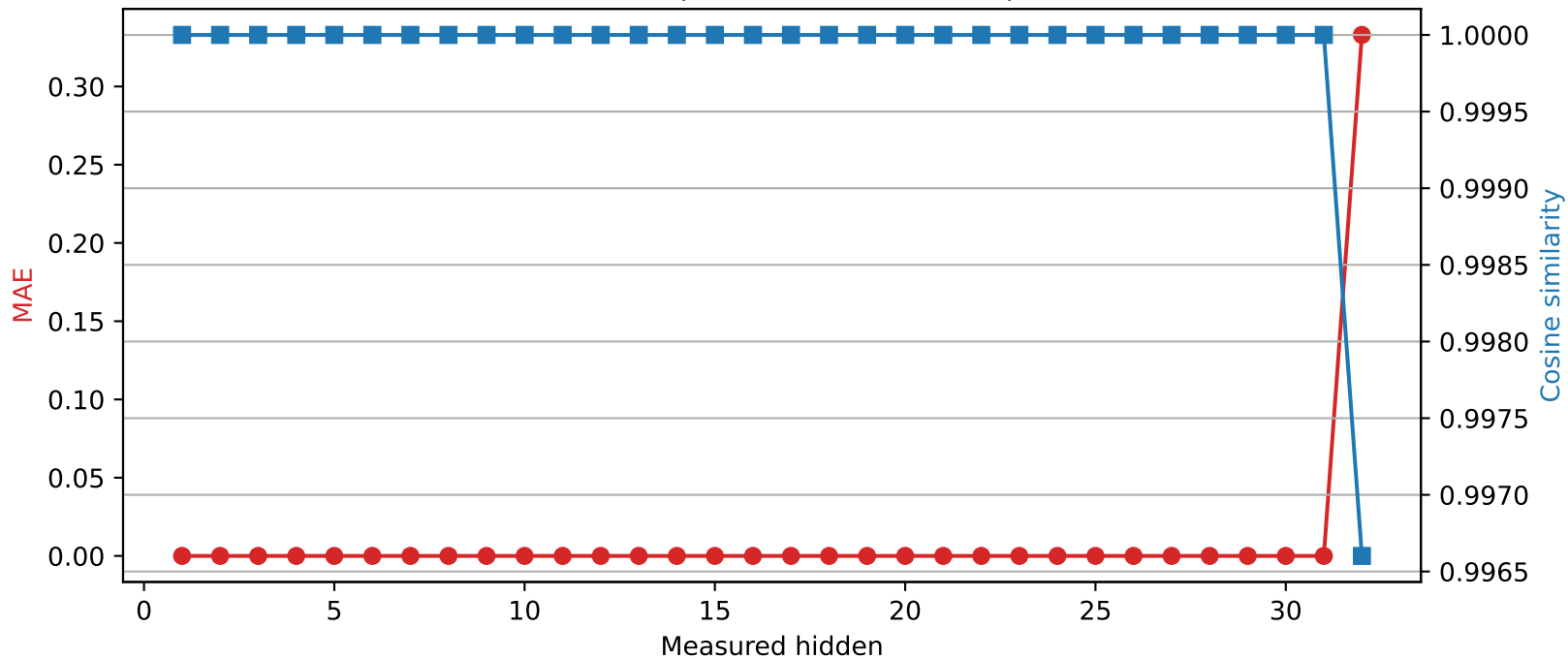
Mistral-7B-Instruct-v0.3 | Quantized layer 31 | float32 → int8
