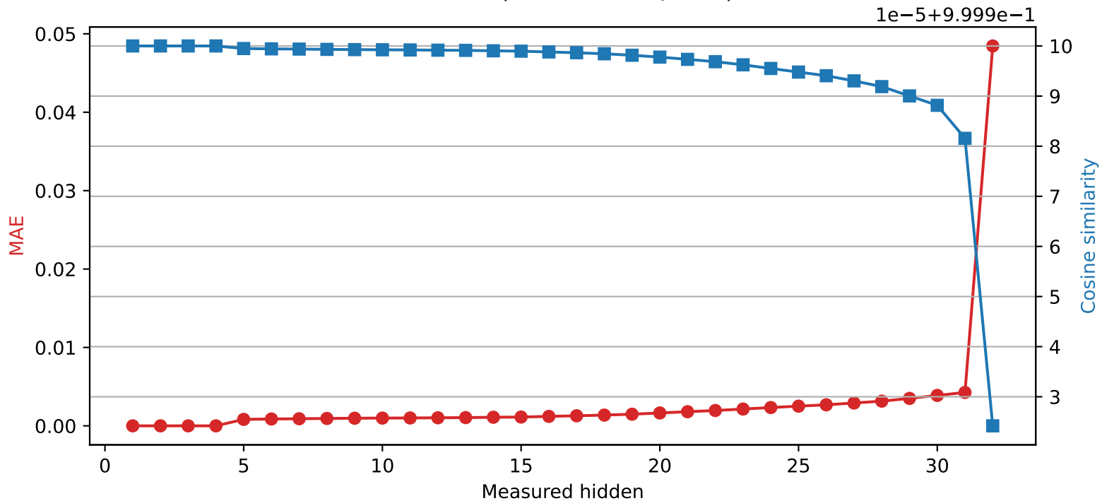
Mistral-7B-Instruct-v0.3 | Quantized layer 4 | float32 → int8
