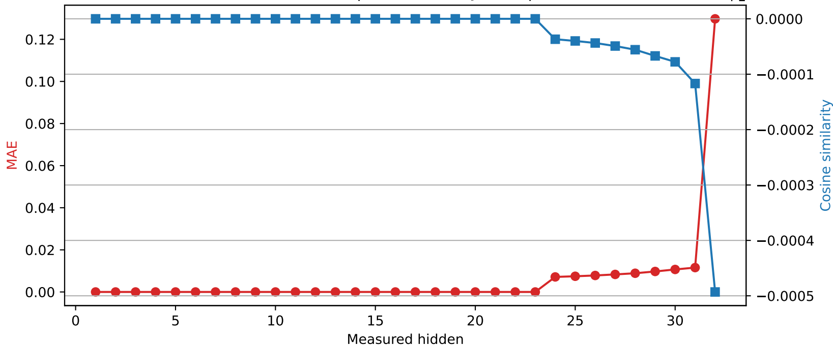
Mistral-7B-Instruct-v0.3 | Quantized layer 23 | float32 → int8
