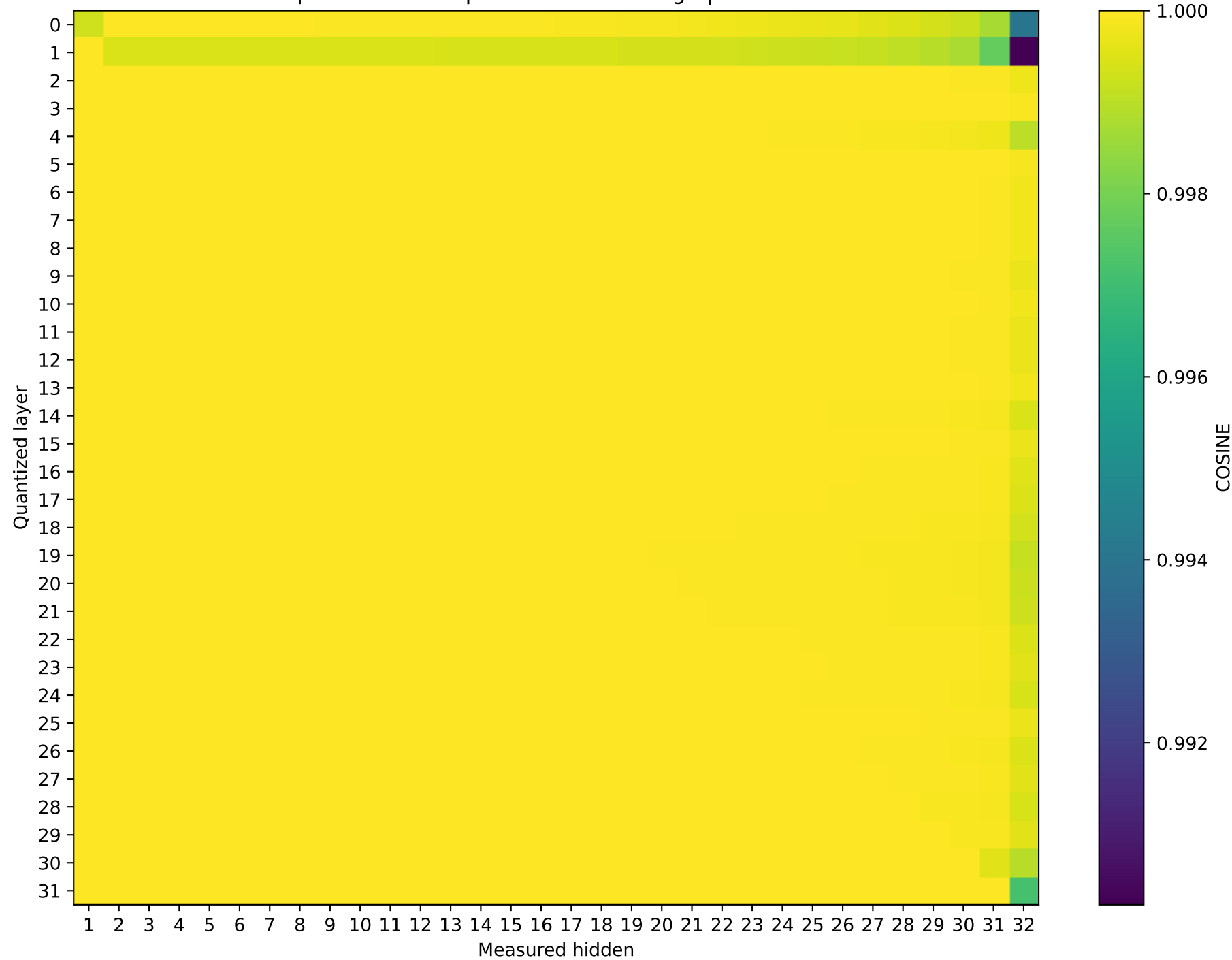
Mistral-7B-Instruct-v0.3 Prompt 3: cos sim representation damage | float32 → int8
