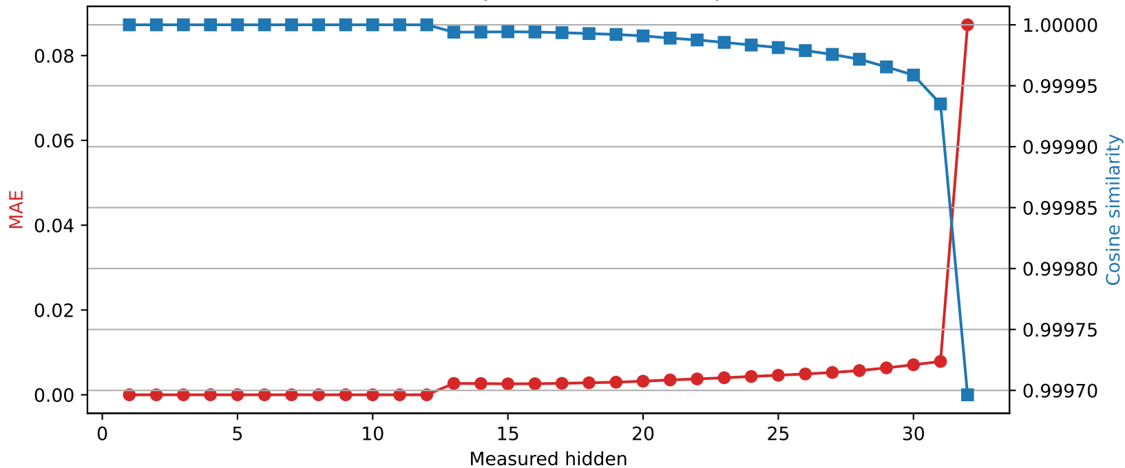
Mistral-7B-Instruct-v0.3 | Quantized layer 12 | float32 → int8
