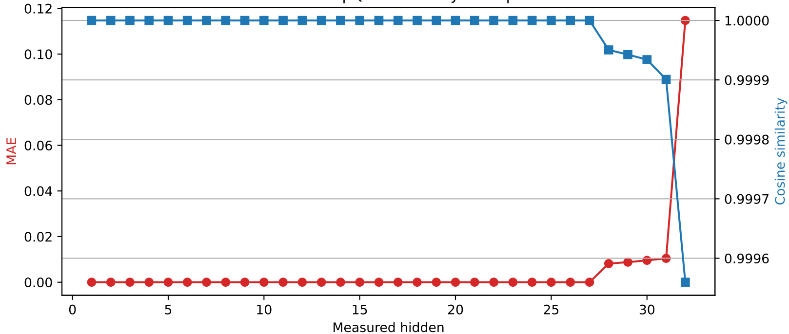
Mistral-7B-Instruct-v0.3 | Quantized layer 27 | float32 → int8
