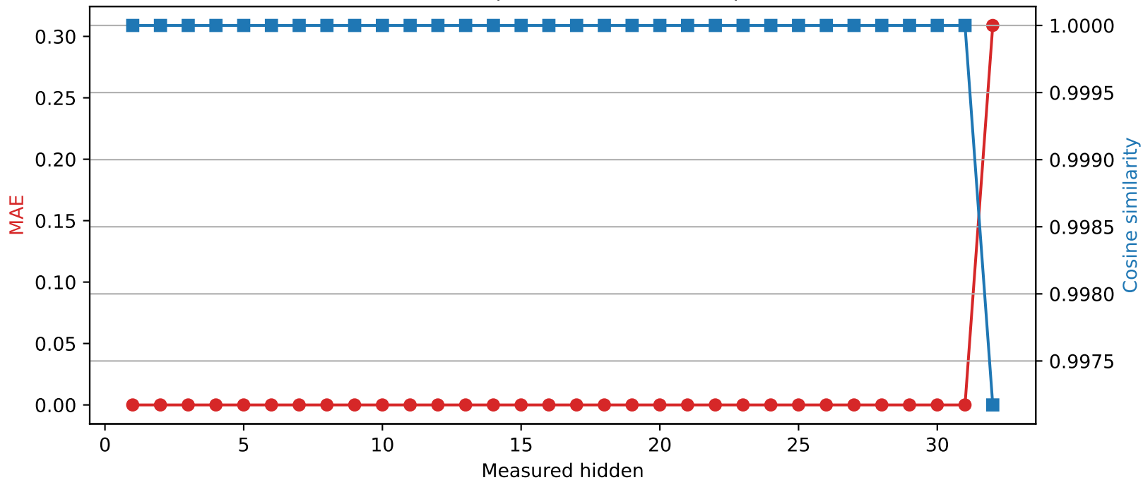
Mistral-7B-Instruct-v0.3 | Quantized layer 31 | float32 \rightarrow int8
