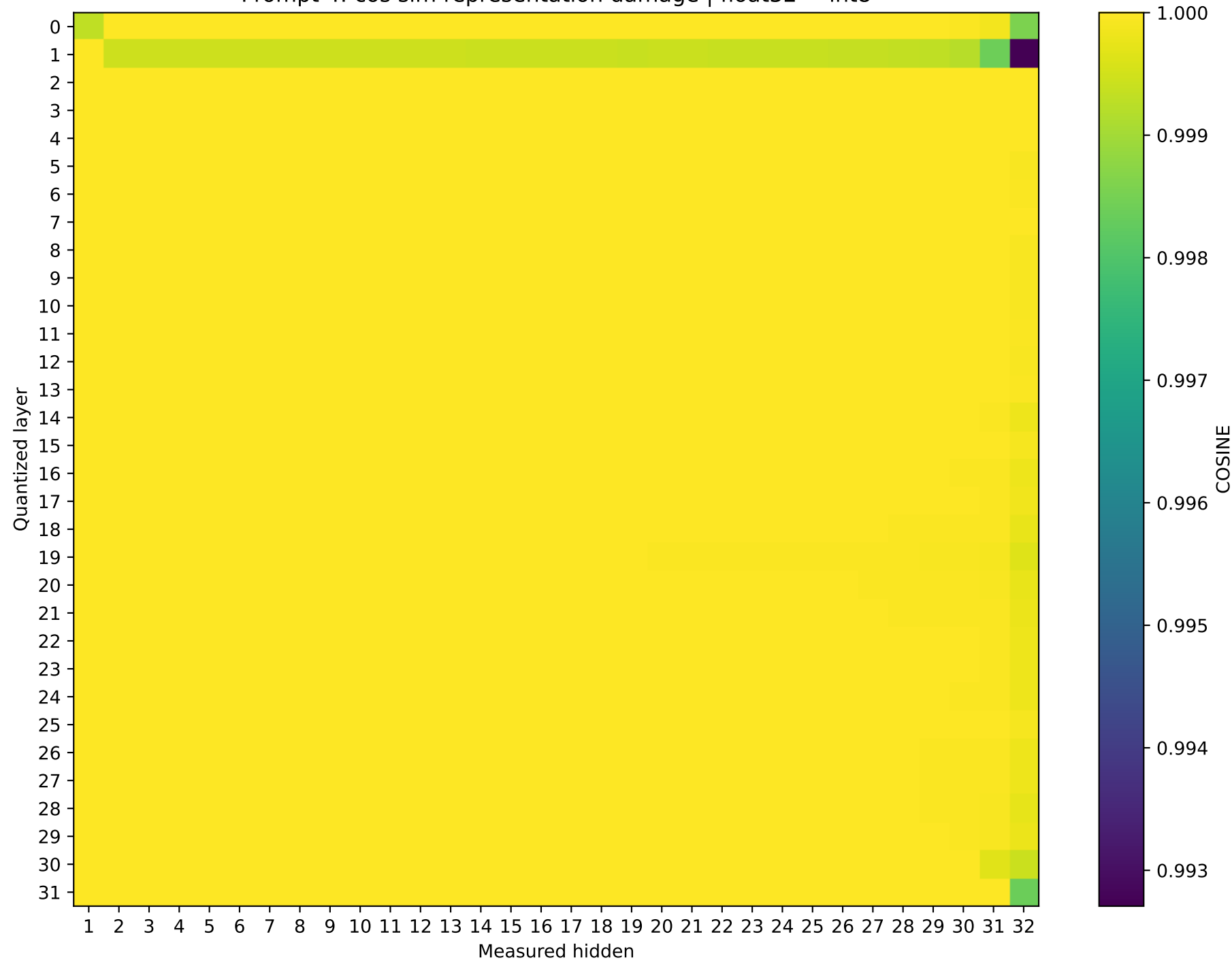
Mistral-7B-Instruct-v0.3 Prompt 4: cos sim representation damage | float32 → int8
