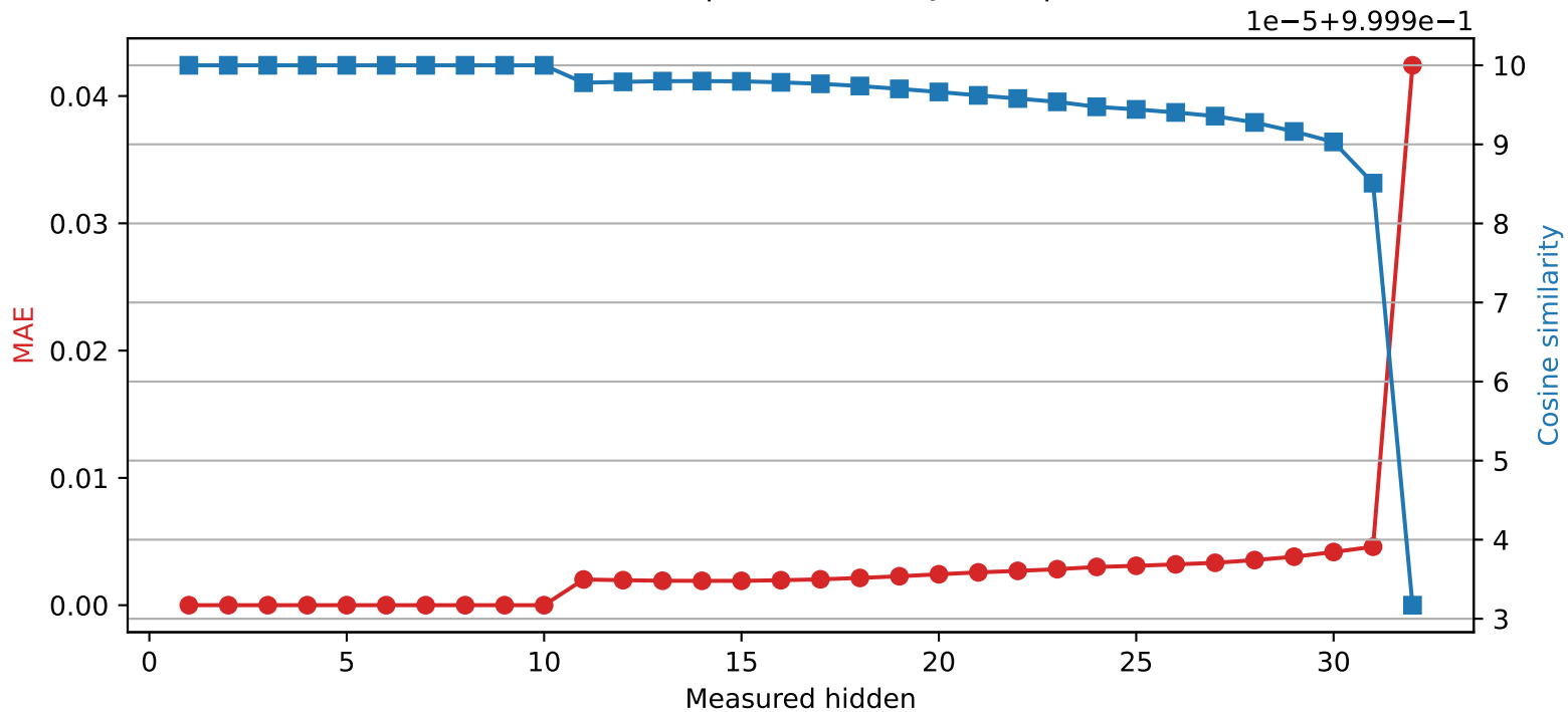
Mistral-7B-Instruct-v0.3 | Quantized layer 10 | float32 → int8
