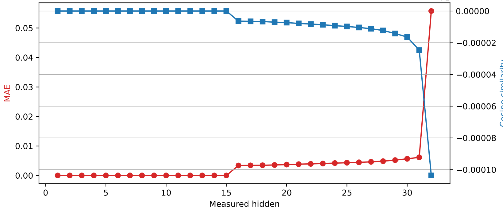
Mistral-7B-Instruct-v0.3 | Quantized layer 15 | float32 → int8
