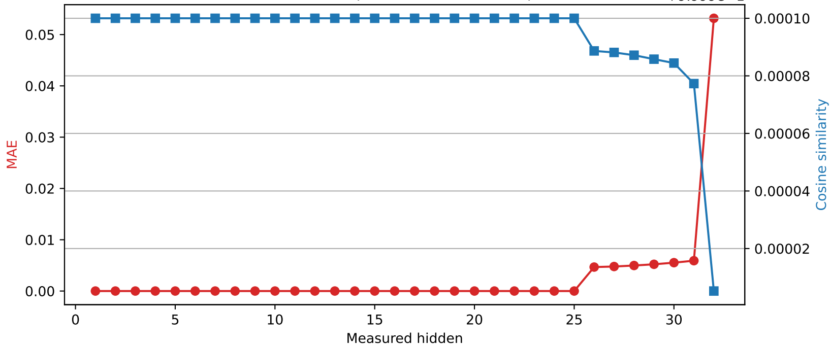
Mistral-7B-Instruct-v0.3 | Quantized layer 25 | float32 \rightarrow int8 +9.999e-1
