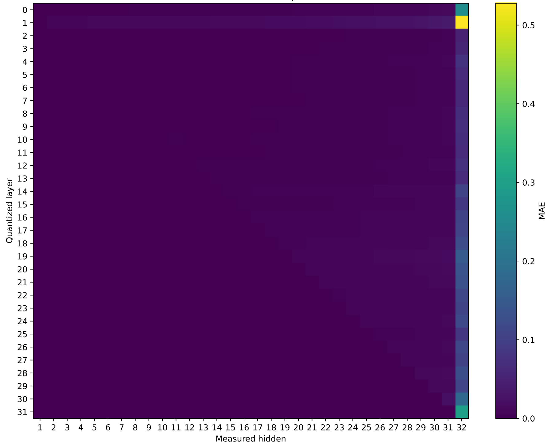
Model: Mistral-7B-Instruct-v0.3 | float64 → int8
