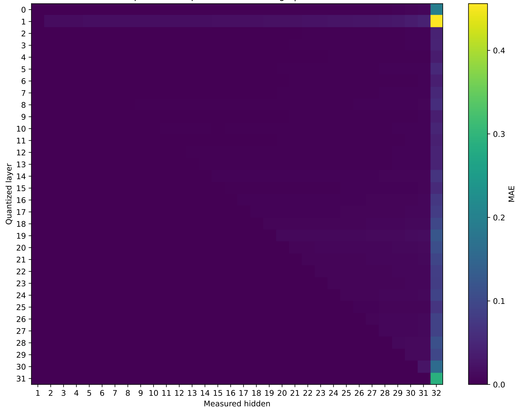
Mistral-7B-Instruct-v0.3 Prompt 0: MAE representation damage | float64 → int8
