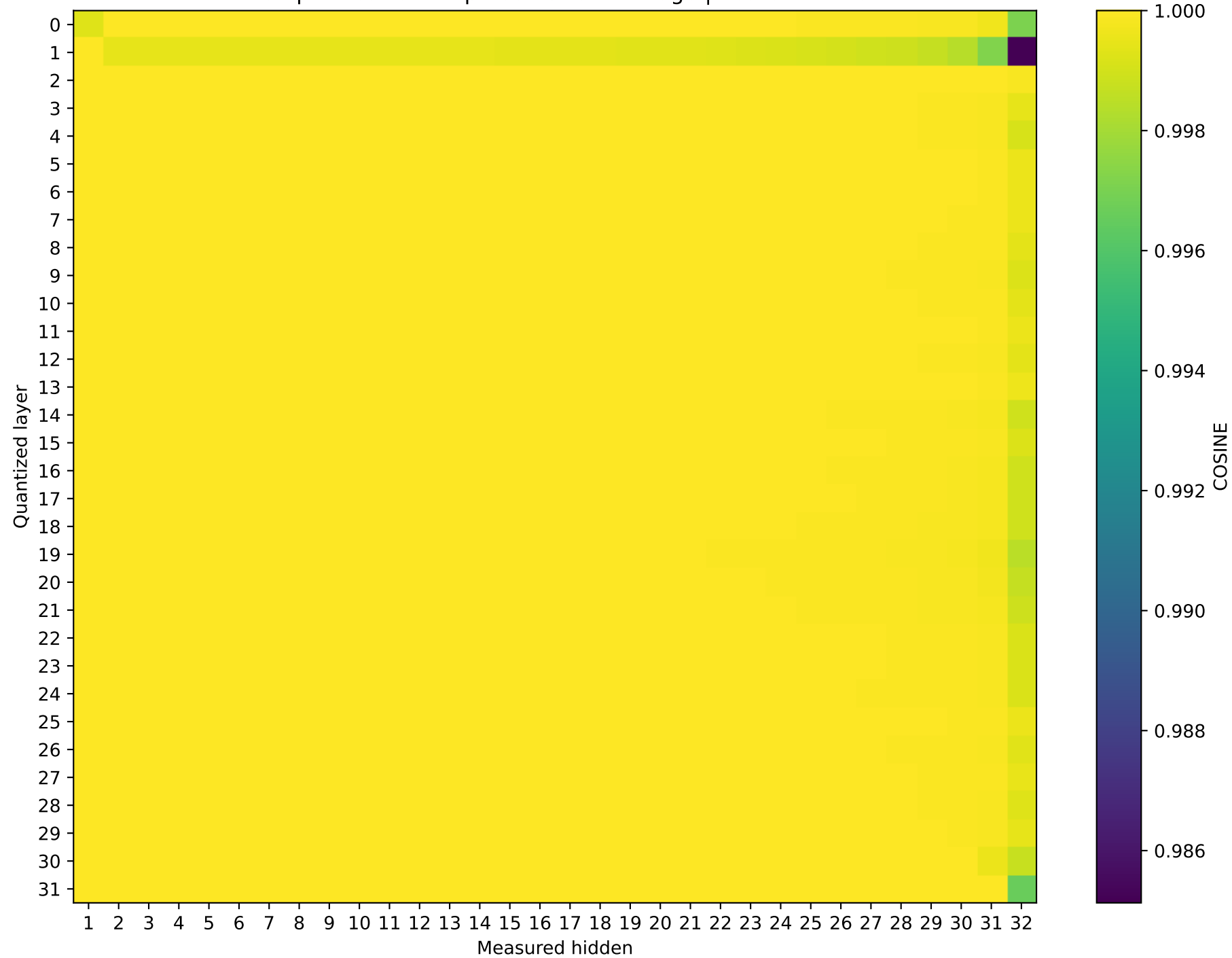
Mistral-7B-Instruct-v0.3 Prompt 1: cos sim representation damage | float64 → int8
