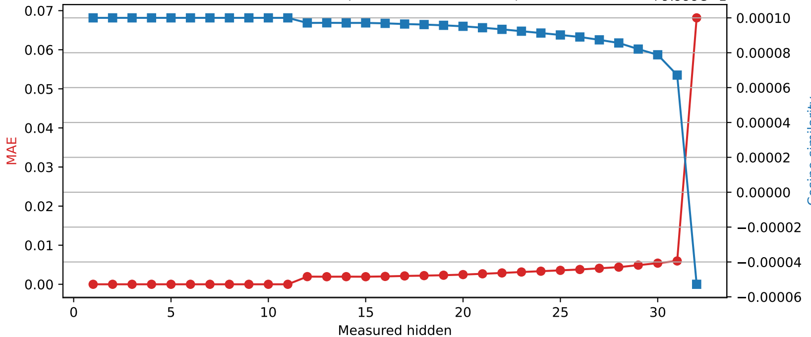
Mistral-7B-Instruct-v0.3 | Quantized layer 11 | float64 → int8 +9.999e-1
