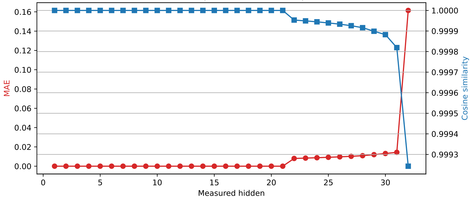
Mistral-7B-Instruct-v0.3 | Quantized layer 21 | float64 → int8
