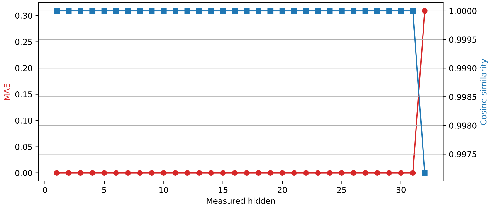
Mistral-7B-Instruct-v0.3 | Quantized layer 31 | float64 → int8
