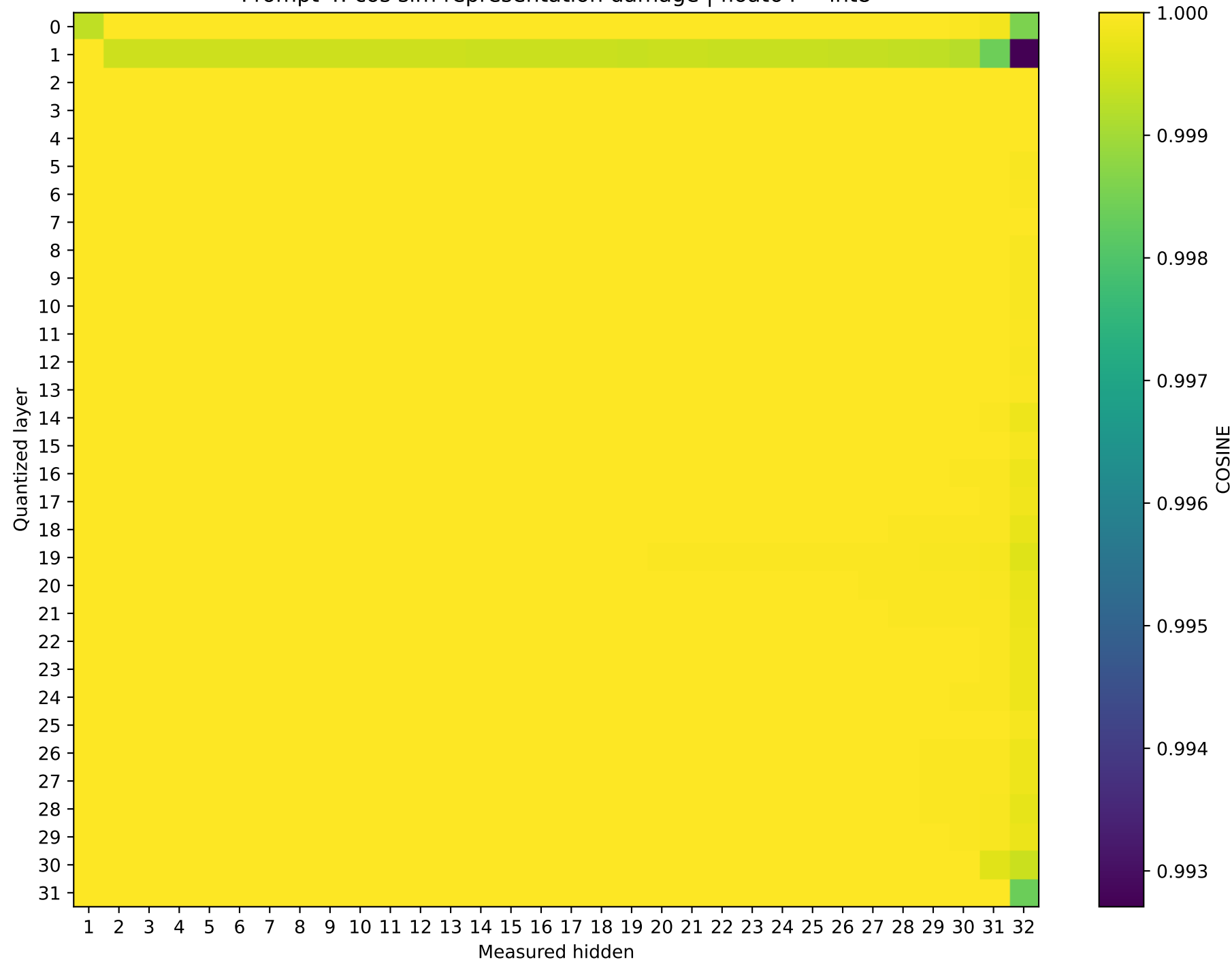
Mistral-7B-Instruct-v0.3 Prompt 4: cos sim representation damage | float64 → int8
