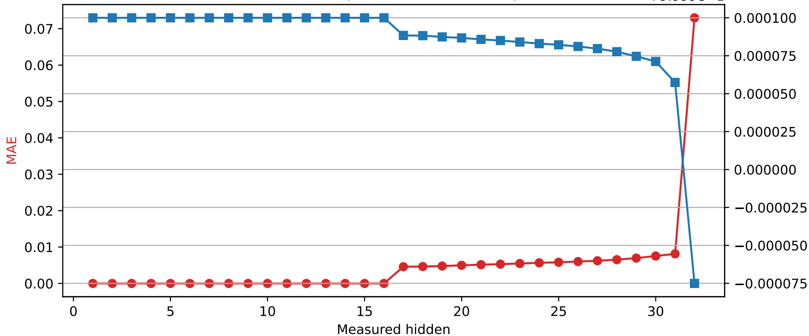
Mistral-7B-Instruct-v0.3 | Quantized layer 16 | float64 → int8 +9.999e-1
