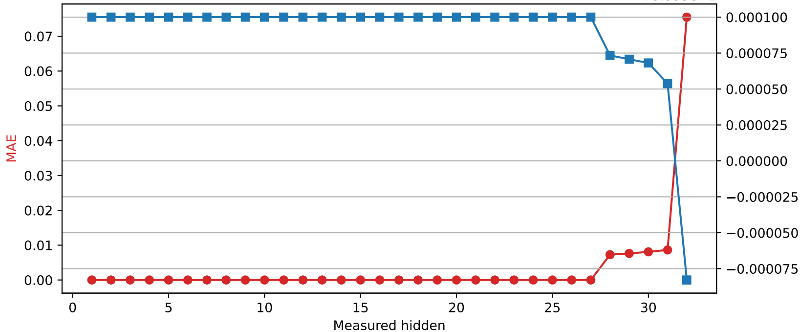
Mistral-7B-Instruct-v0.3 | Quantized layer 27 | float64 → int8 +9.999e-1
