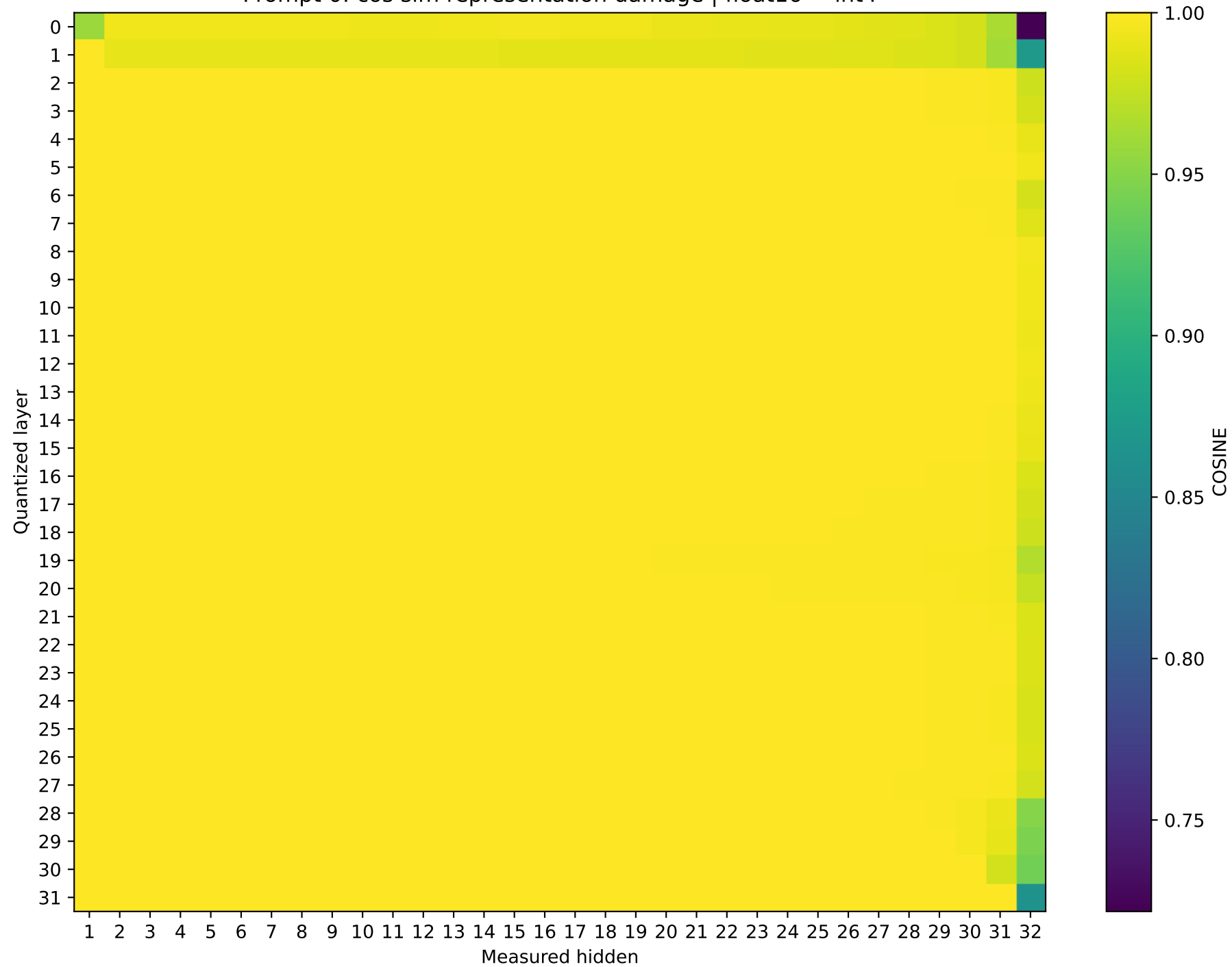
Mistral-7B-Instruct-v0.3 Prompt 0: cos sim representation damage | float16 \rightarrow int4
