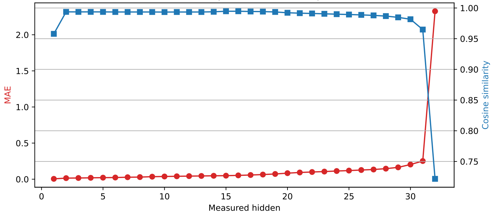
Mistral-7B-Instruct-v0.3 | Quantized layer 0 | float16 → int4
