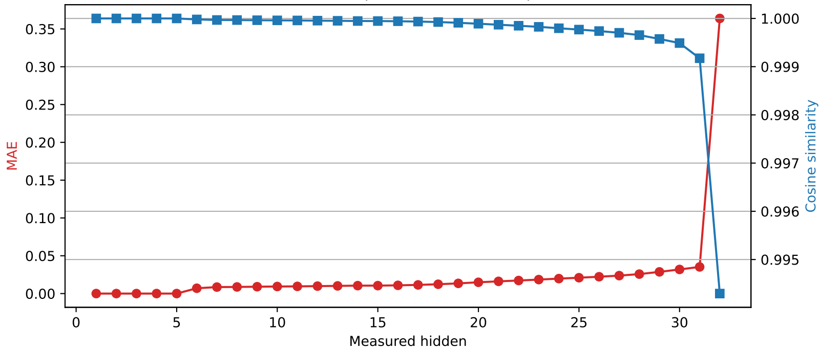
Mistral-7B-Instruct-v0.3 | Quantized layer 5 | float16 \rightarrow int4
