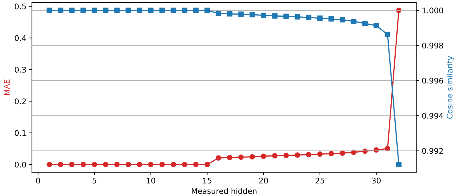
Mistral-7B-Instruct-v0.3 | Quantized layer 15 | float16 \rightarrow int4
