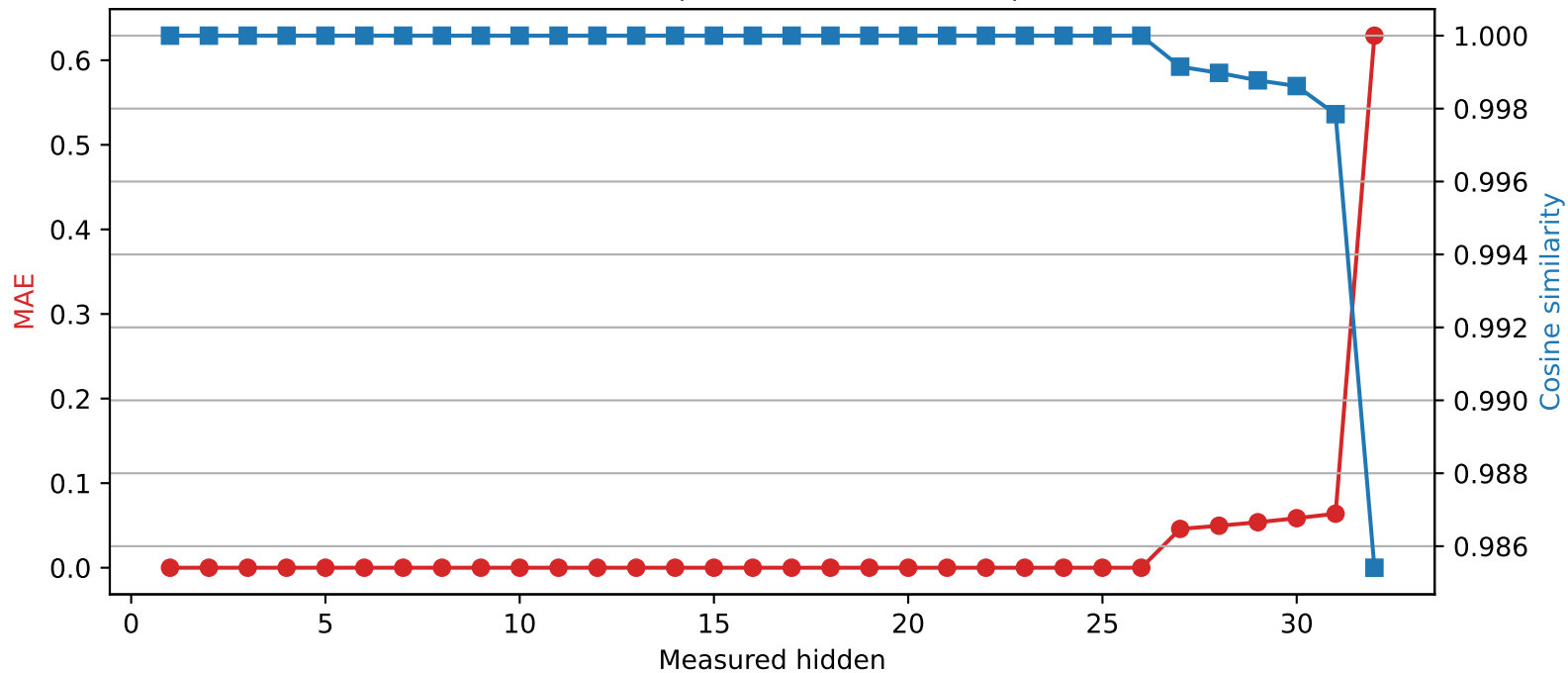
Mistral-7B-Instruct-v0.3 | Quantized layer 26 | float16 \rightarrow int4
